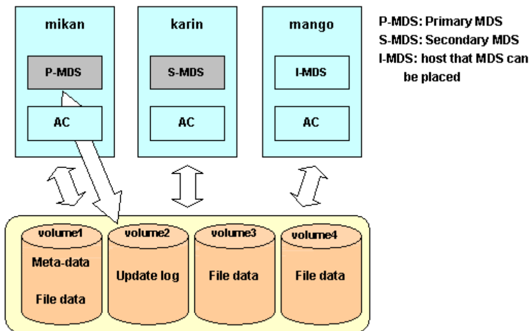
Figure Separating the update log area and multiple file data partitions configuration
