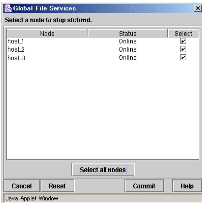
Figure [Operate]: [Operate sfcrmd]:[Stop] Screen
