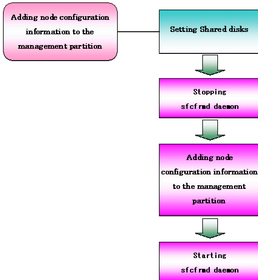
Figure Operation flow for addition node configuration information to the management partition
